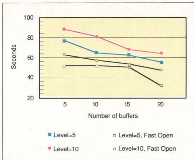
Figure 5: The performance improvements from using 20 Fast Open caches. The test copied files from an N-level-deep subdirectory to another N-level-deep subdirectory for 10 iterations, where N is 5 or 10 and each subdirectory contains five 32K-byte files.
